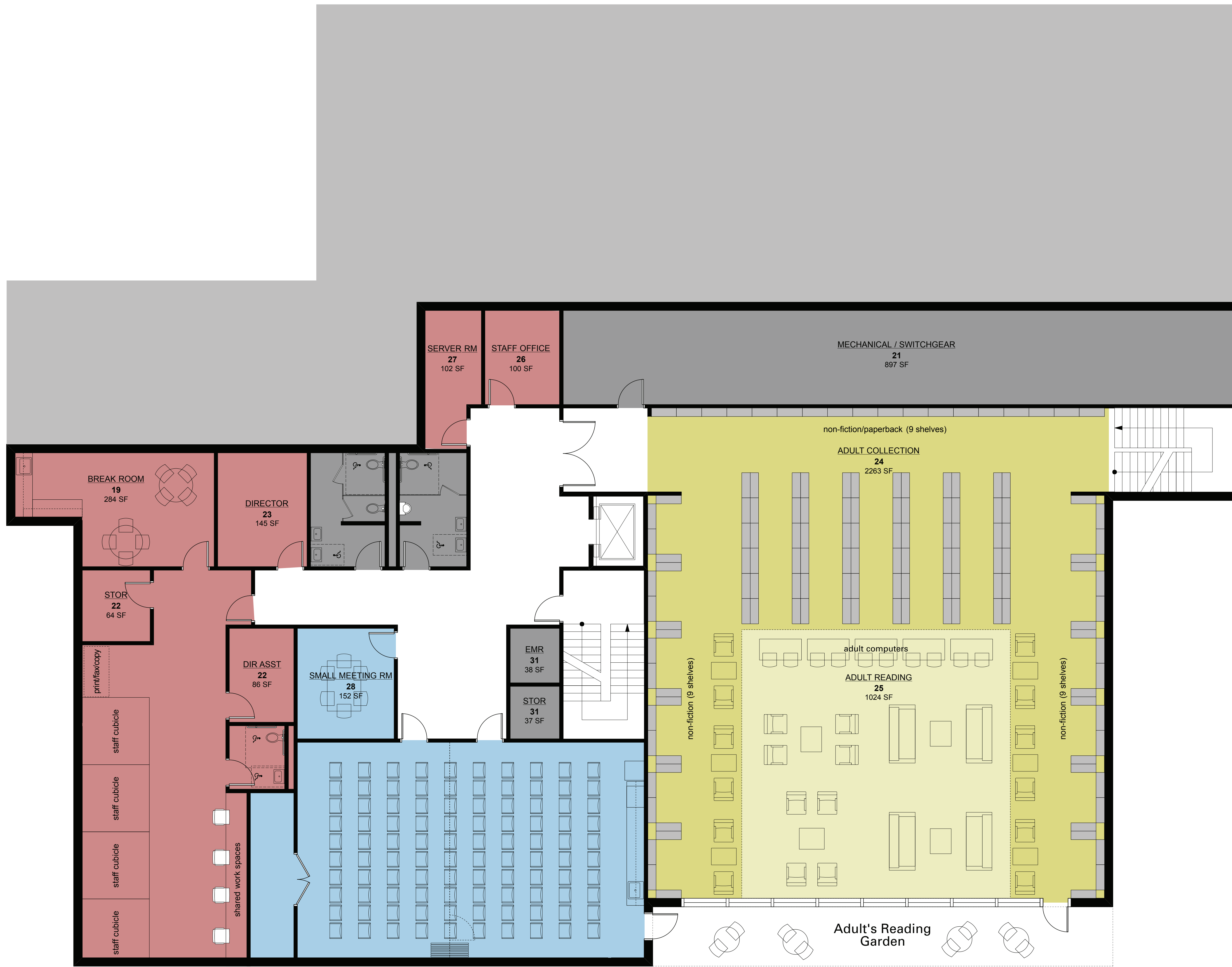
FLOOR PLAN - LOWER LEVEL 0 10 20 30 FT
